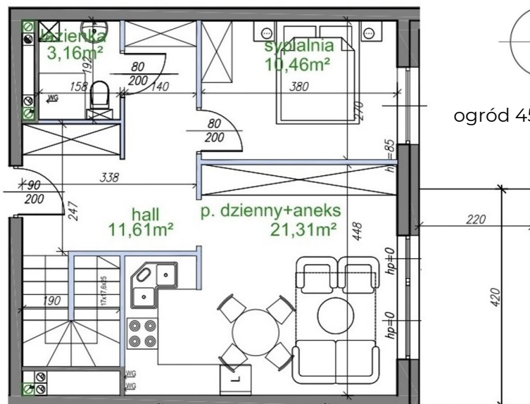
PARTER
